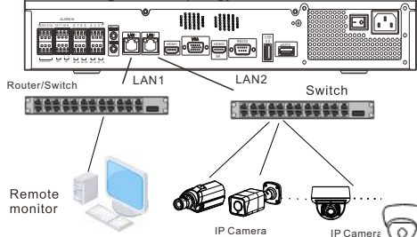
Figure 4-3 Topology of the NVR
