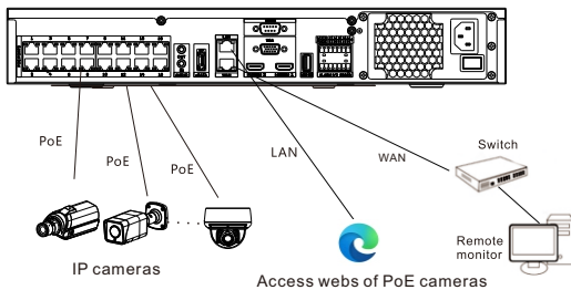
Figure 4-3 Topology of the NVR
