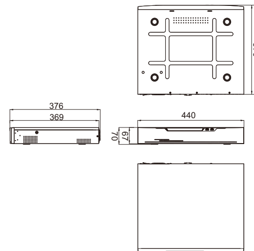
Figure 2-1 Dimensions (Unit:mm)
