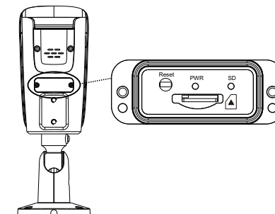
Figure 2-3 Install SD card
