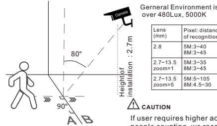
Figure 4-5 Installation of people counting
